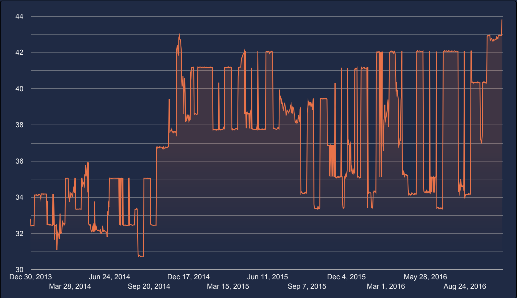
Sales Price Per Unit Over Time
