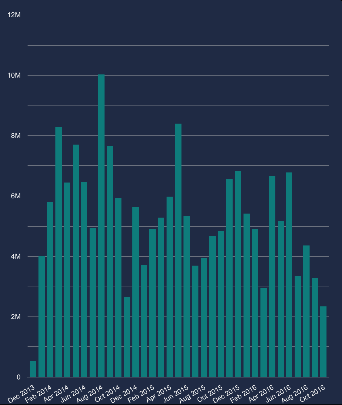
Sales by Month of Year
