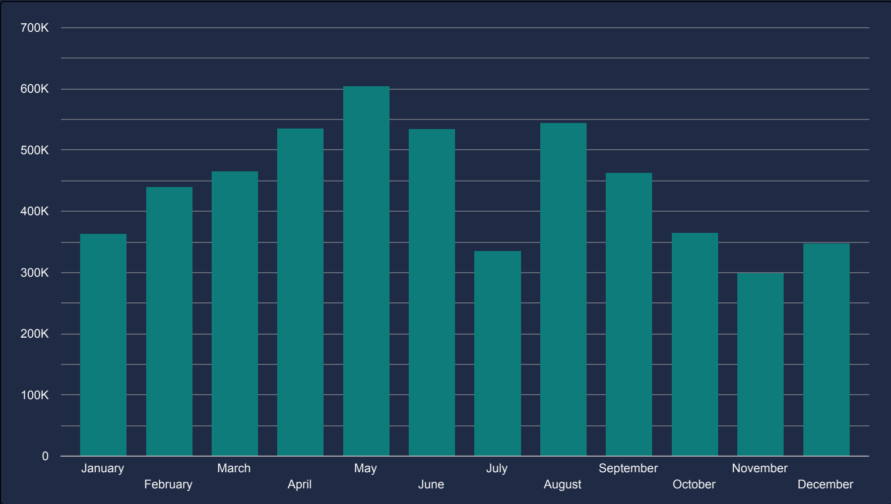
Quantity Sold by Month of Year
