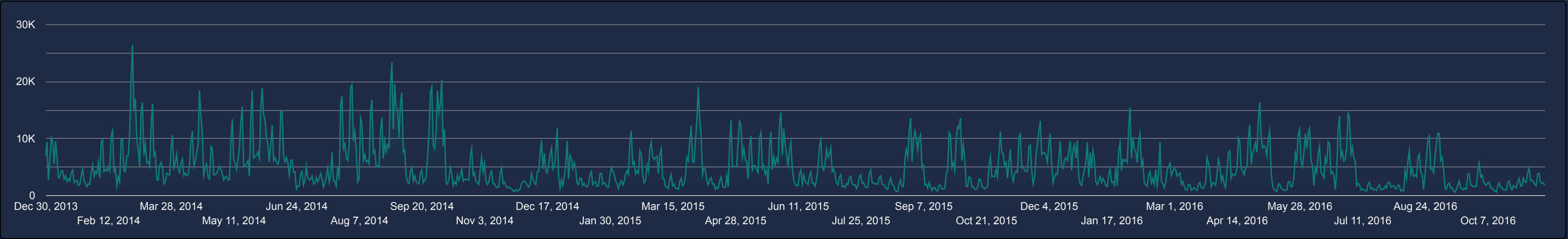
Quantity Sold Over Time
