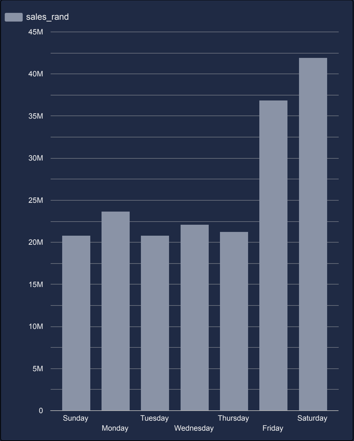
Sales by Day of the Week
